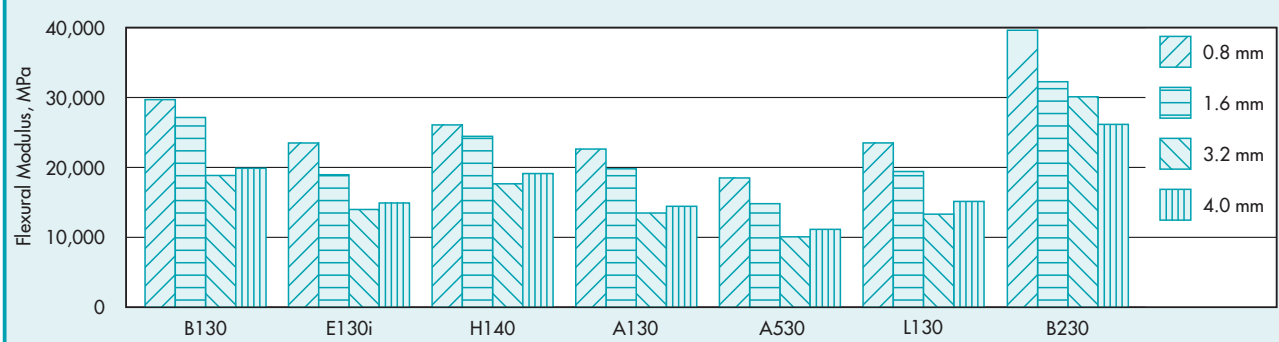
Fig. 3.1.5 • Flexural Modulus versus Wall Thickness Vectra LCP
