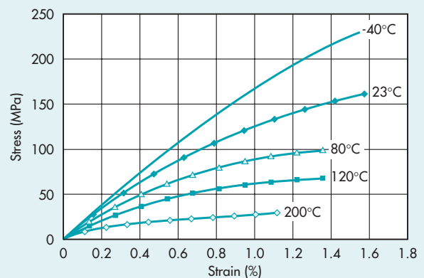
Fig. 3.1.8b · Influence of Temperature on Stress Strain Behavior, Vectra E130i
