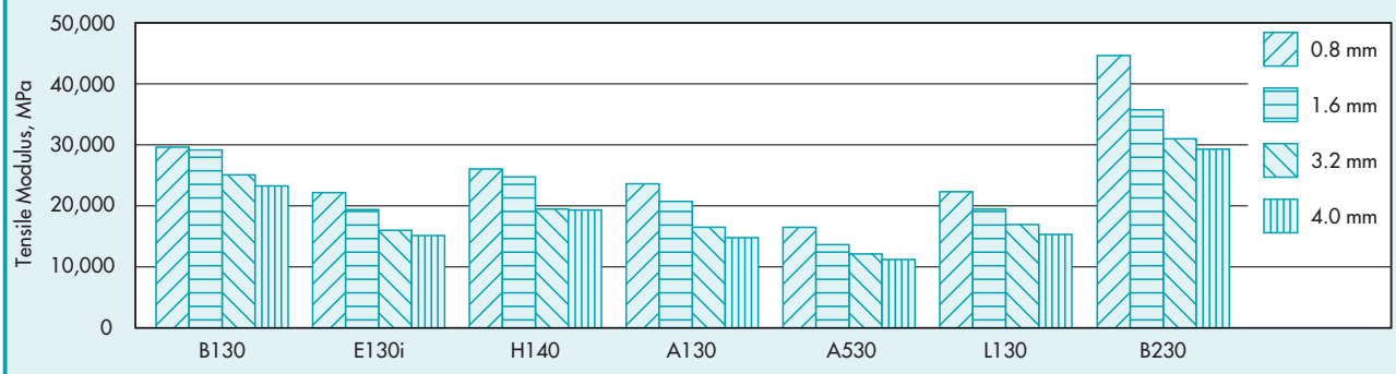
Fig. 3.1.3 • Tensile Modulus versus Wall Thickness Vectra LCP
