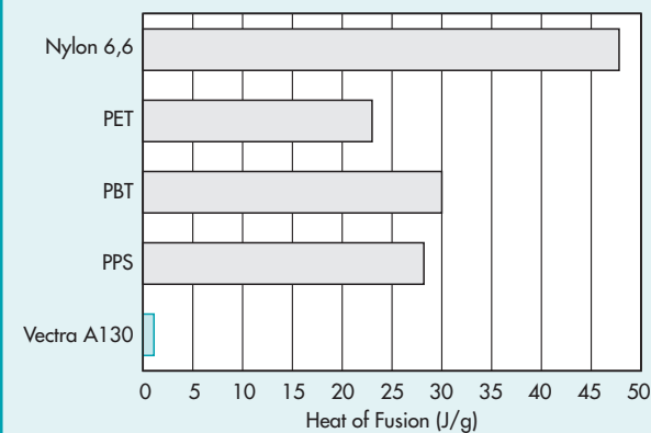
Fig. 3.2.12 • Relative Phase Transition Energy
