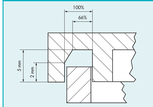
Fig. 10.2.3 • Spin Welding Joint Design
