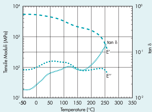
Fig. 3.2.2 • Dynamic Mechanical Analysis Vectra A530
