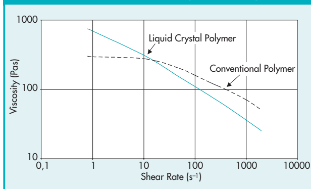
Fig. 8.1 • Melt Viscosity Comparison Vectra® LCP versus Semi-Crystalline Polymer
