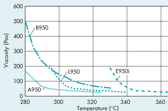
Fig. 8.3 • Melt Viscosity versus Temperature (Unfilled grades at shear rate = 1,000/s)
