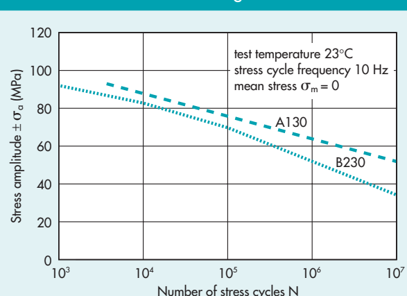
Fig. 3.1.17 · Wöhler Curves for Vectra, longitudinal direction determined in the alternating flexural stress range
