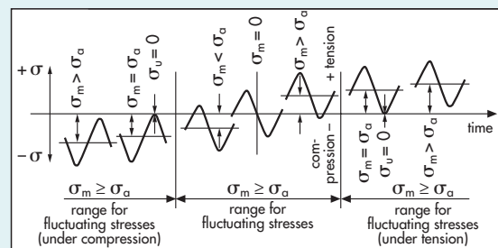
Fig. 3.1.16 · Stress Ranges in Fatigue Tests
