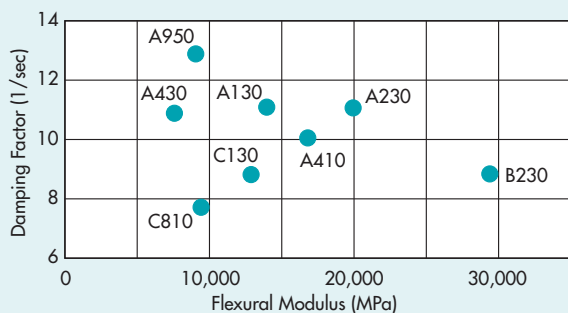
Fig. 3.1.20 • Vibration Characteristics
