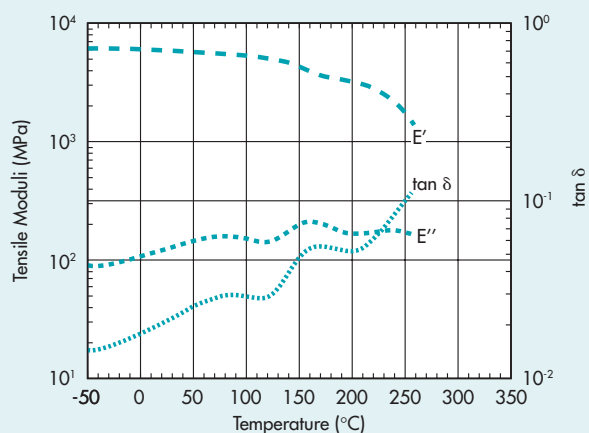
Fig. 3.2.4 • Dynamic Mechanical Analysis Vectra B230
