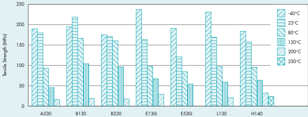
Fig. 3.1.10 • Tensile Strength versus Temperature, Vectra LCP
