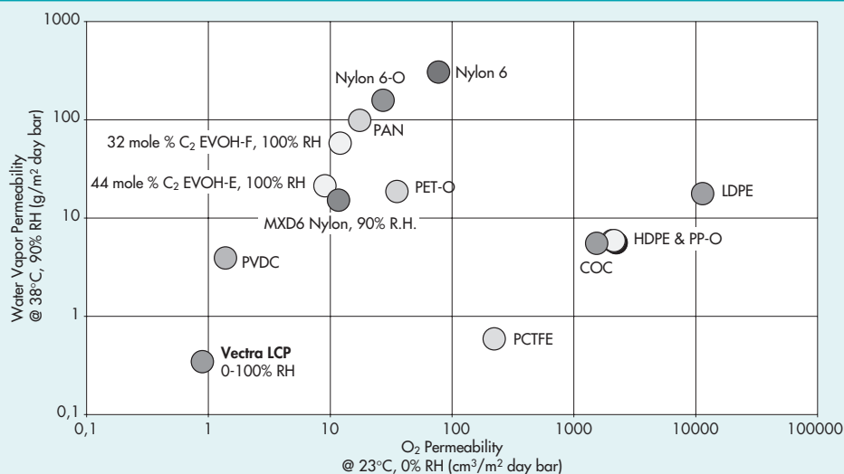
Fig. 4.3.1 · Permeability of Various Polymer Films (Thickness 25µm)
