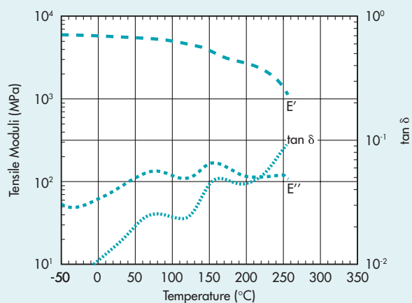
Fig. 3.2.3 • Dynamic Mechanical Analysis Vectra B130
