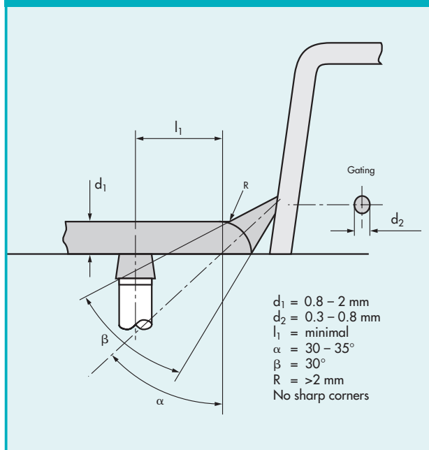
Fig. 9.2.2 • Submarine Gate
