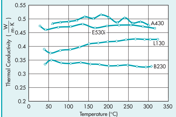
Fig. 3.2.14 • Thermal Conductivity
