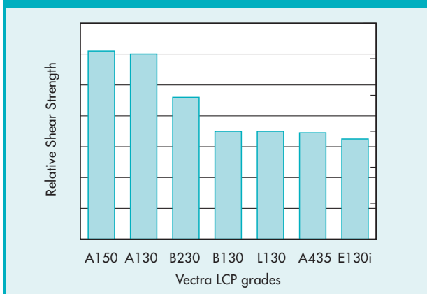
Fig. 10.2.2 • Ultrasonic Weld Strengths
