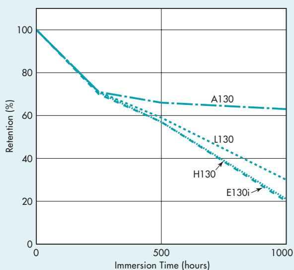
Fig. 4.1.1 • Tensile Strength versus Immersion Time in Hot Water (120°C, 2 bar)
