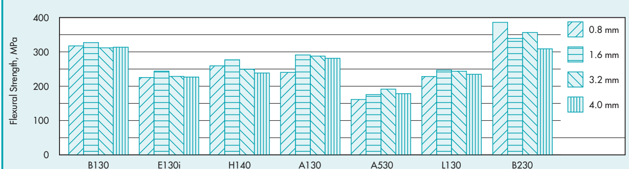
Fig. 3.1.6 • Flexural Strength versus Wall Thickness Vectra LCP
