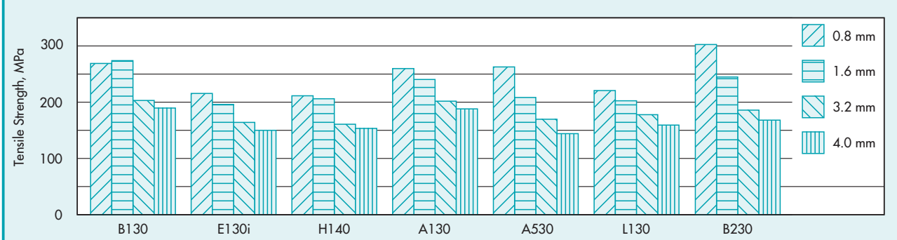
Fig. 3.1.4 • Tensile Strength versus Wall Thickness Vectra LCP
