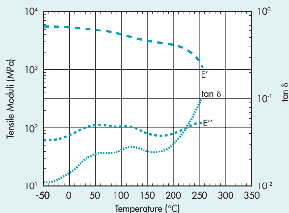
Fig. 3.2.1 • Dynamic Mechanical Analysis Vectra A130
