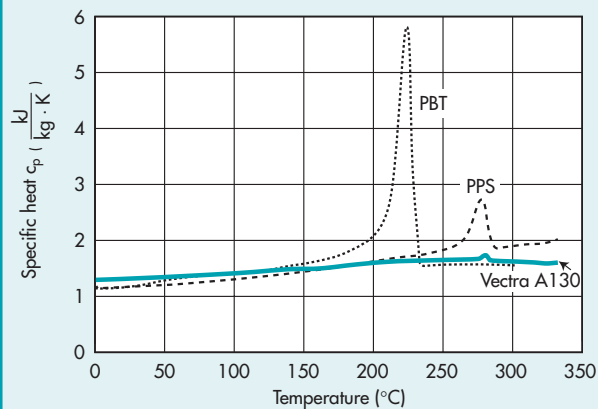
Fig. 3.2.11 • Specific Heat
