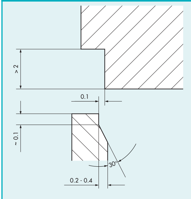
Fig. 10.2.1 • Ultrasonic Welding Joint Design
