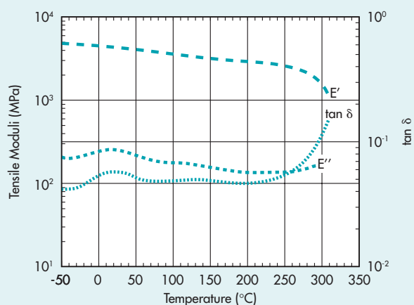
Fig. 3.2.5 • Dynamic Mechanical Analysis Vectra E130i
