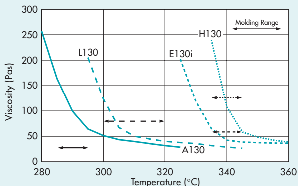
Fig. 8.2 • Melt Viscosity versus Temperature (Glass filled grades at shear rate = 1,000/s)
