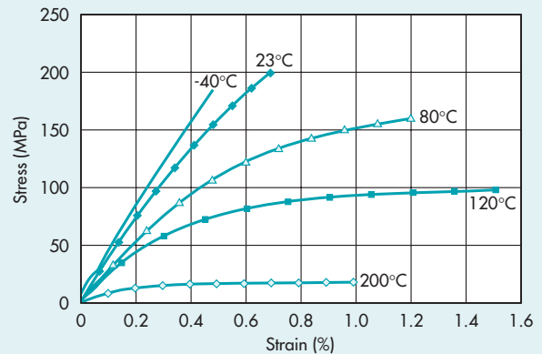
Fig. 3.1.8a · Influence of Temperature on Stress Strain Behavior, Vectra B230
