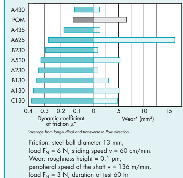
Fig. 3.1.18 • Friction and Wear
