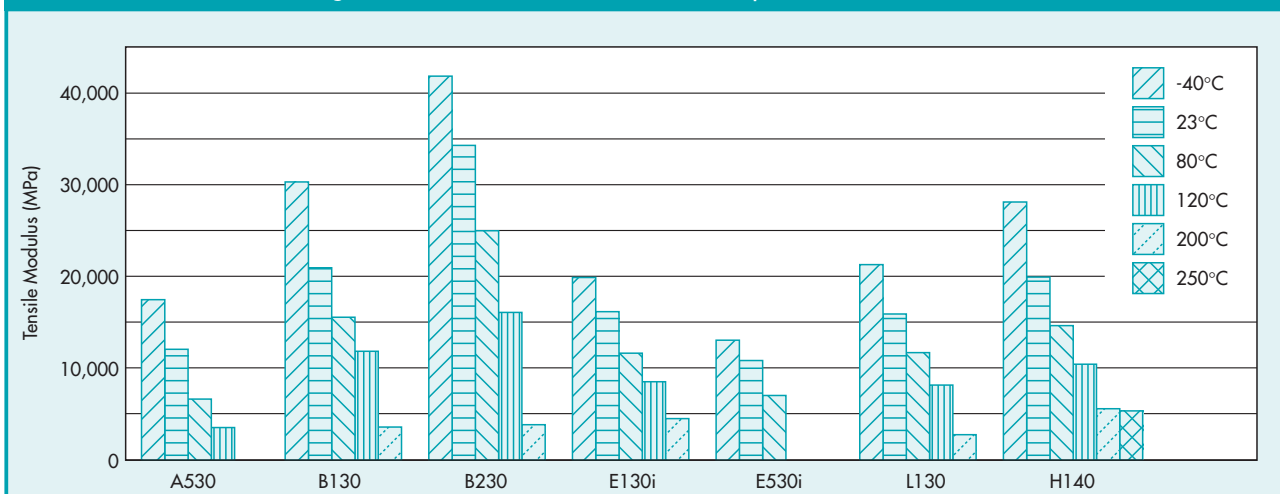
Fig. 3.1.9 · Tensile Modulus versus Temperature, Vectra LCP
