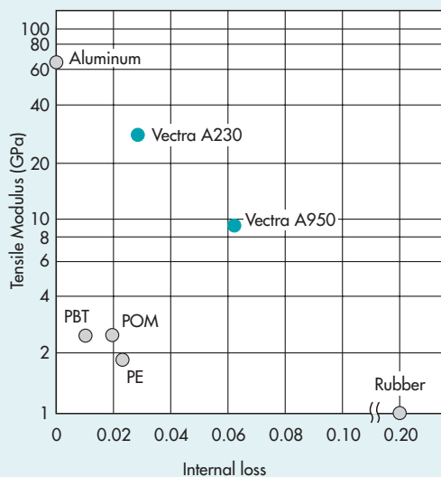
Fig. 3.1.19 • Damping Properties
