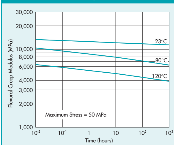
Fig. 3.1.15 · Flexural Creep Modulus, Vectra C130
