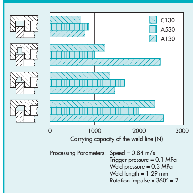
Fig. 10.2.4 • Spin Weld Strengths for Vectra® LCP
