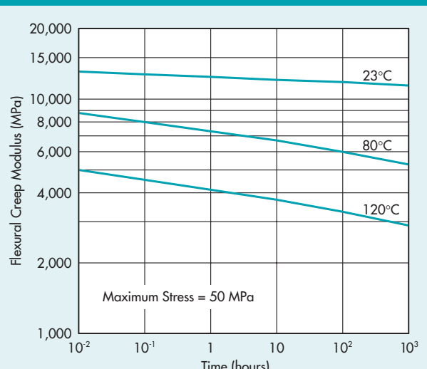
Fig. 3.1.13 • Flexural Creep Modulus, Vectra A130
