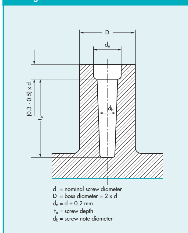
Fig. 10.2.7 · Boss for EJOT PT® K Screw
